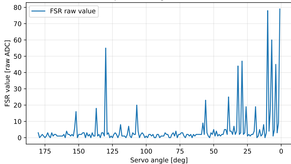
FSR response during servo movement
